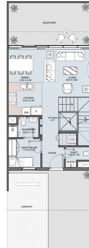
GROUND FLOOR Middle Unit
